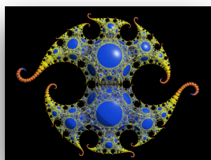
Jos Leys 2007 1 on 15 cusp
