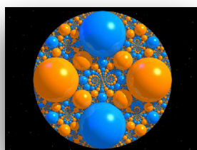
Jos Leys 2007 1 on 15 cusp
