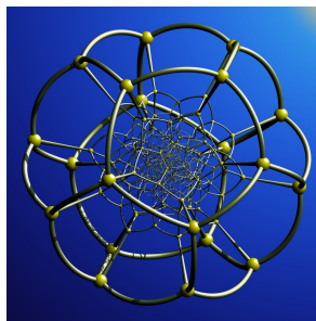
Dodecahedral tessellation of the hypersphere https://www.josleys.com/show_gallery.php?galid=379
