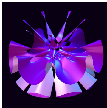
O. Labs. Septic de Labs
