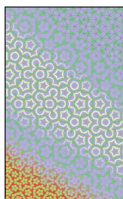
Penrose II. D. Austin - W. Casselman - D.Wright
