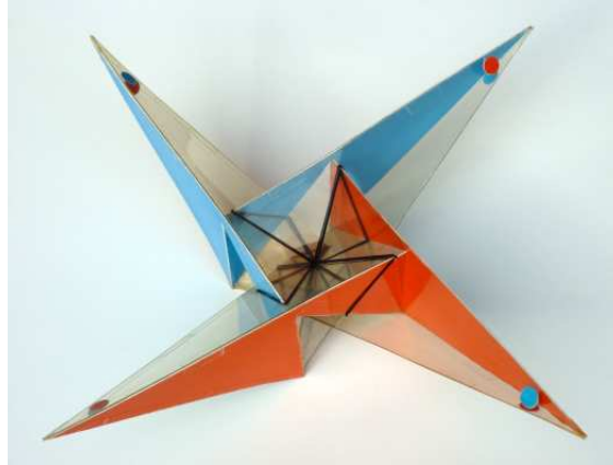
Fig. 9 Open halfway model: handmade models need ability, precision and perseverance. The pentagons are obtained by gluing together two cardboard sheets – one side in red for the one and one side in blue for the other. To work the rhodoïd, a steel edge and a fine cutter are necessary. To mark the rhodoïd from the plans, needles and a small hammer were used. Faces are fixed together with adhesive tape. The self-intersection line is drawn by using a pencil with permanent ink.
