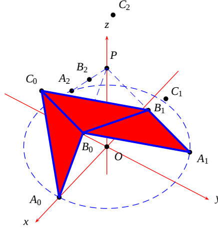
Fig. 1 The pentagonal face P_0 and its triangulation. Note that the three triangles in red are isosceles and have an angle which measure is 120^\circ . Simple and nice! During the deformation the pentagons can be folded along the sides of the triangles. This picture is realized with LaTeX and the packages psticks and pst-3dplot.
