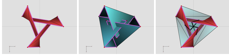
Fig. 2 Construction of the Boy surface by gluing together a Möbius strip and a disk.
