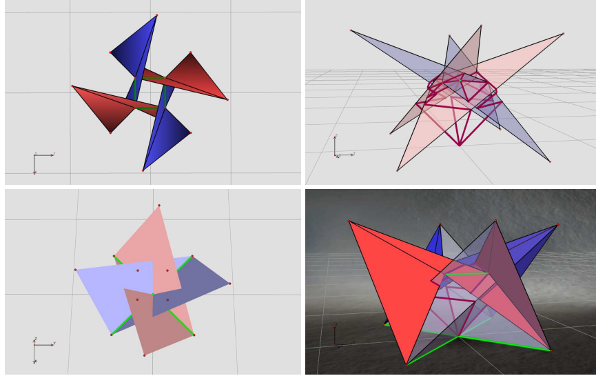
Fig. 11 Closed halfway-model; decomposition in different geometries with JavaView. It is useful to locate the two perpendicular edges [A_0A_2] and [A_1A_3] and the square B_0B_1B_2B_3 (in green).
