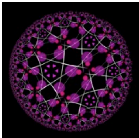
Poincaré Berries
