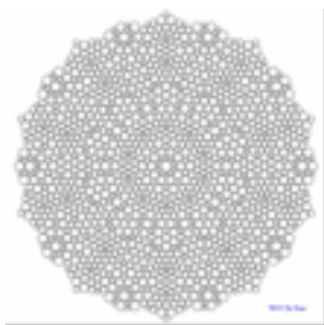
Penrose circles 1
