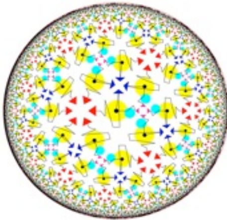
Hyperbolic Klee
