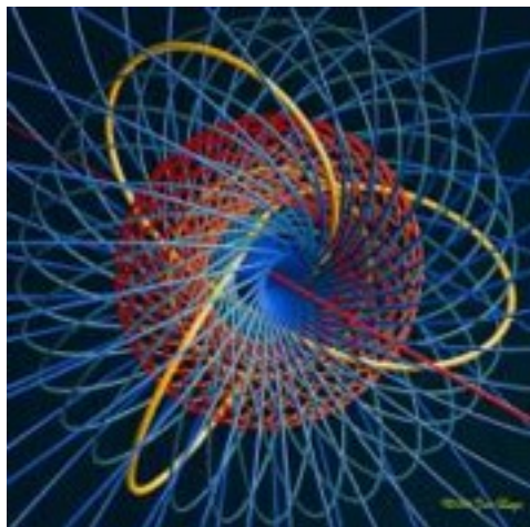
Seifert fibration
