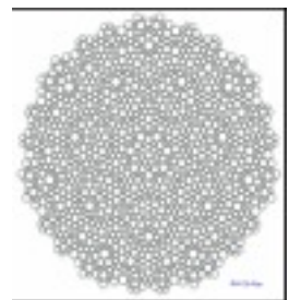
Penrose circles 2
