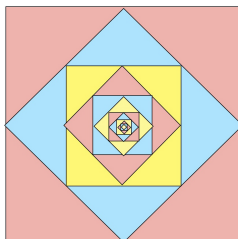
Fig.51: Carré "fractal"
