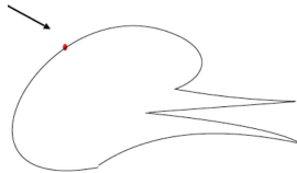
Fig.10: (2,6)-polygone
