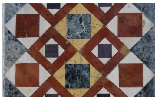
Fig.24: carré 1
