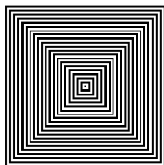
Fig.52: Illusion "carrés"
