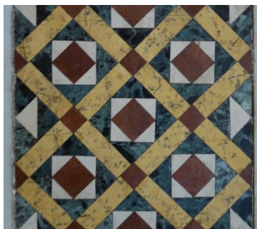
Fig.25: carré 2
