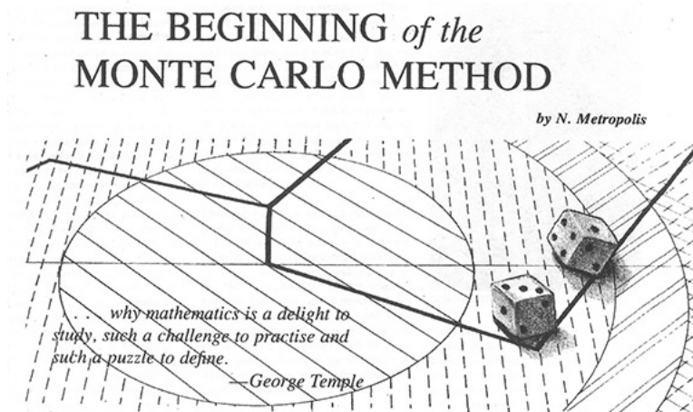
Figure 7.2: Neutron paths and dice on a sketch of a reactor, from N. Metropolis’s article in Los Alamos Science [Met87], by permission Triad National Security LLC.
