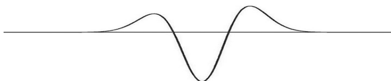
Figure 11.3: The modification of the second derivative of the Gaussian kernel that kills the exponential of y/2 .
