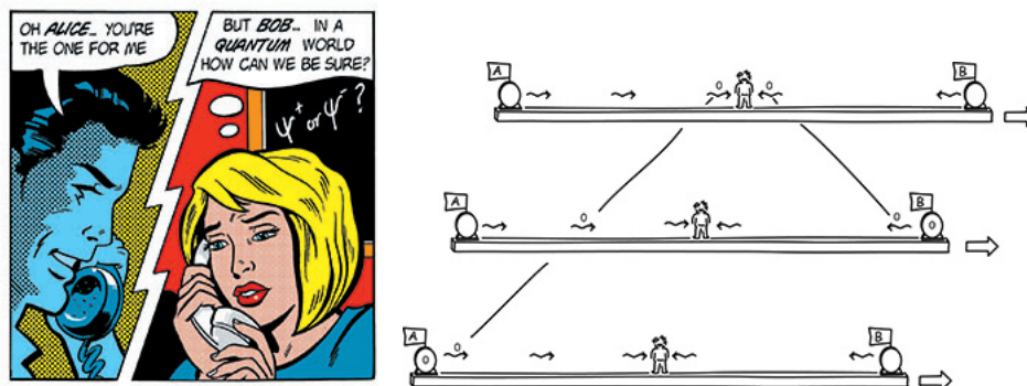
Figure 10.9: On the left: love in a quantum world, image by John Richardson, by permission of IOP publishing; on the right, from lecture notes of Prof. John Norton with his permission, a platform with clocks at each end is moving steadily to the right, an observer in the center watches two clocks A and B. The observer ascribes simultaneity to the times when he receives A and B's signals, times that are not simultaneous to the stationary observer.
